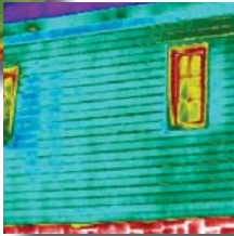
After: The same home with Fullback installed; notice the cool blue color; studs and air leak are no longer visible.
